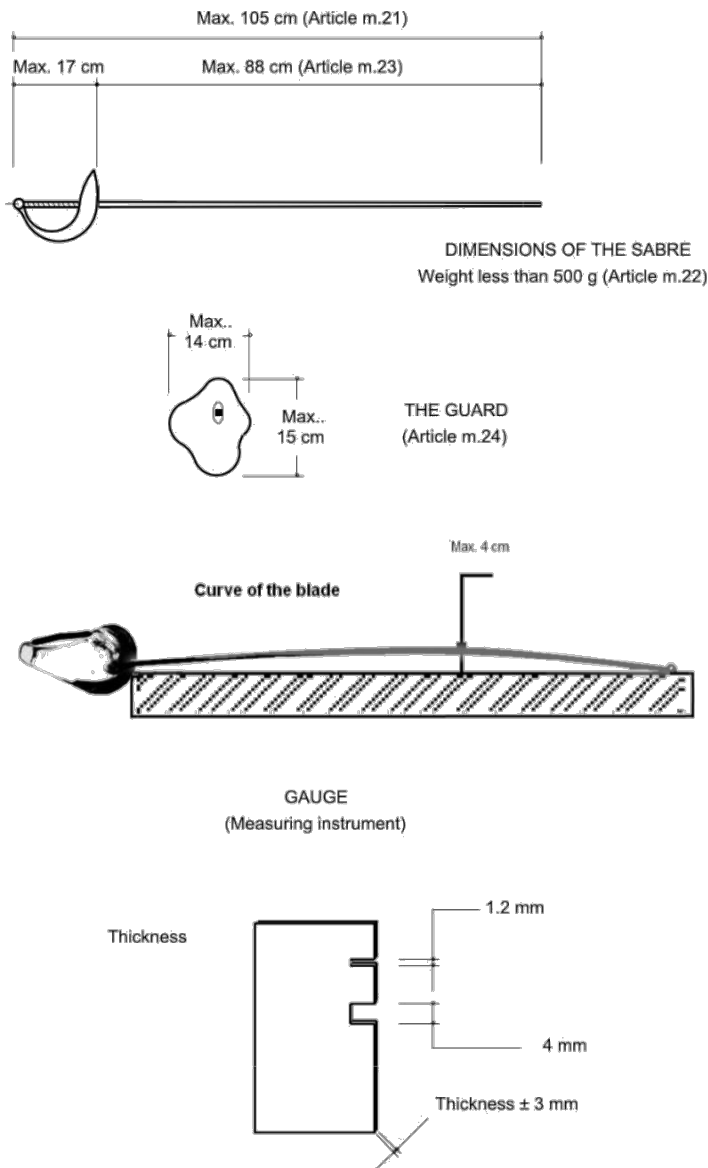
Figure 13. Sabre dimensions (contd.)
